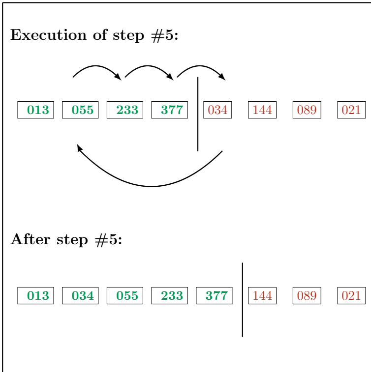
Figure 2.4: Insertion sort.
