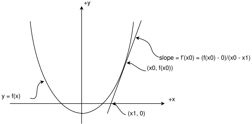
Figure 13.1: Newton's method.
