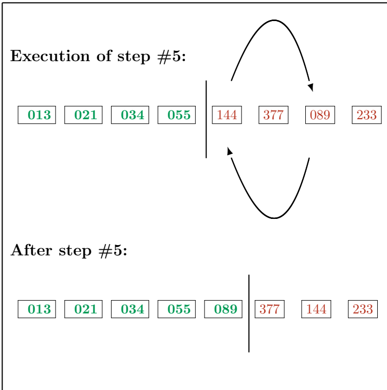
Figure 2.3: Selection sort.
